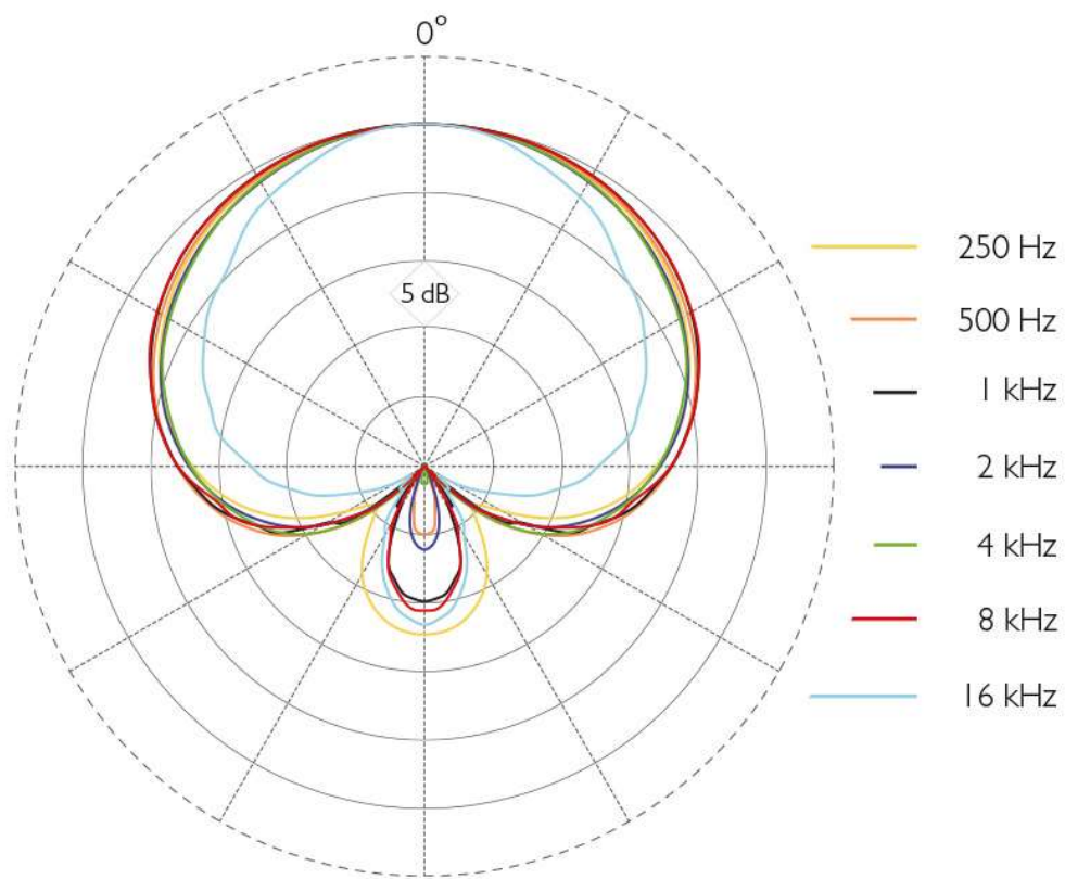
Typical directional characteristics of DPA 4018
