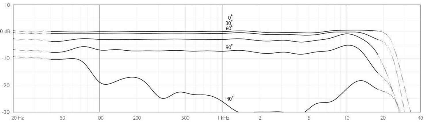
Typical on and off-axis response of DPA 4018
