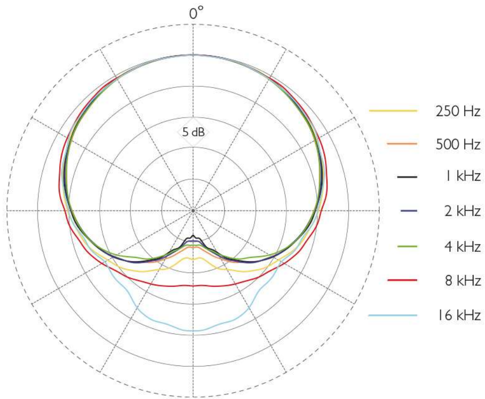
Typical directional characteristics of a 4088
