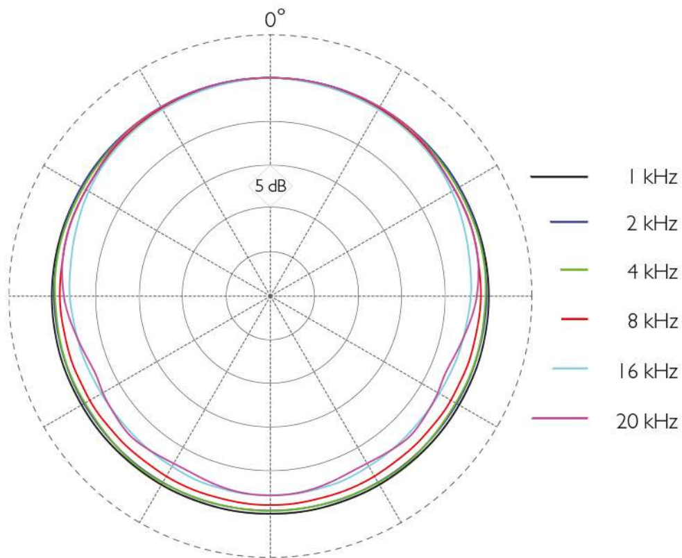
Typical response of a 4063
