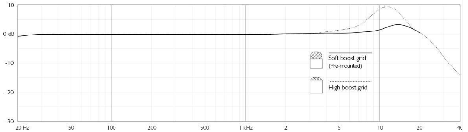
Typical response of a 4063
