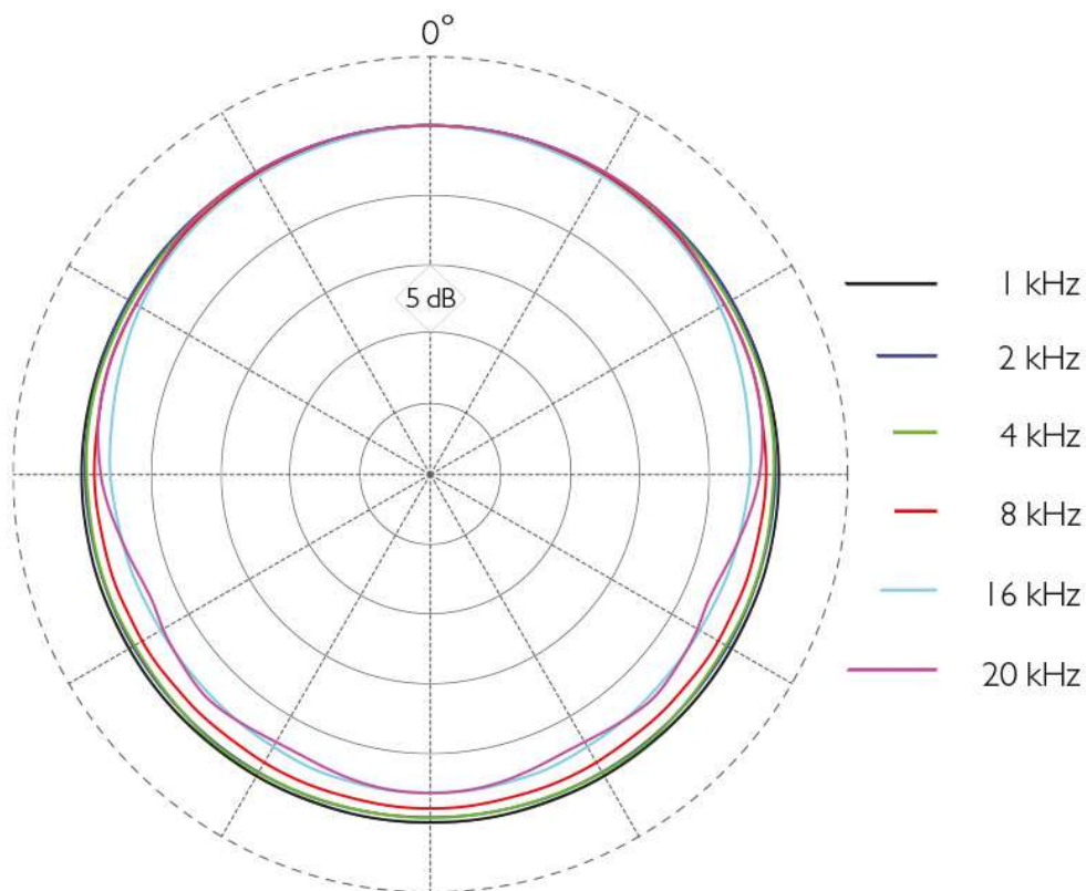
Typical response of a 4061
