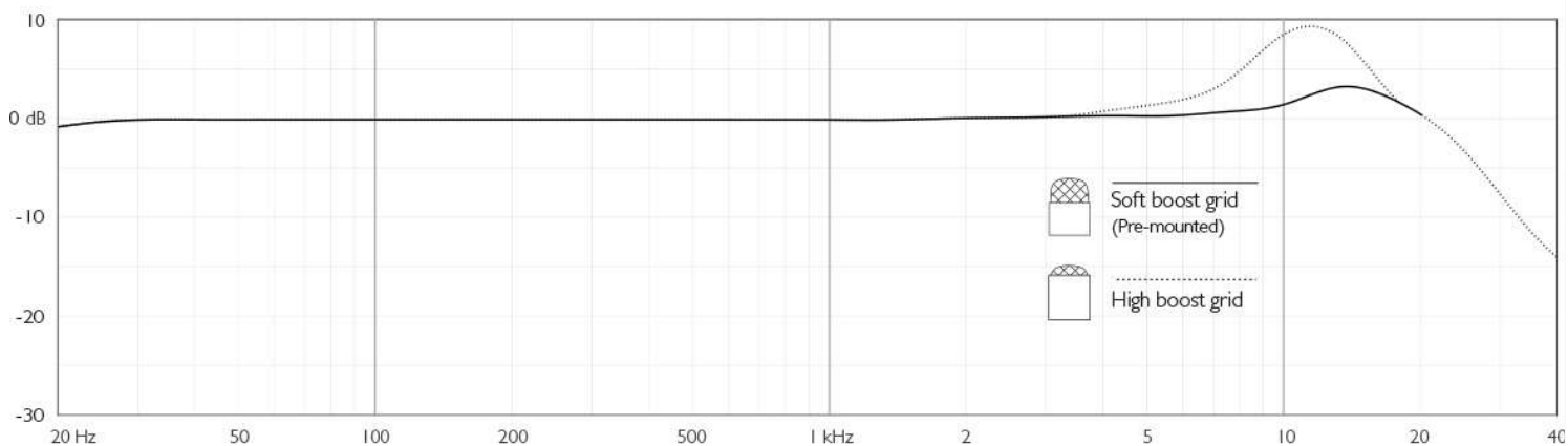
Typical response of a 4061
