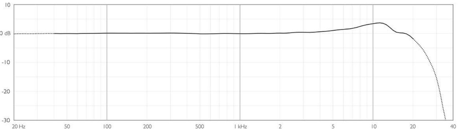
Typical on-axis response of a 2012 measured at 30 cm (11.8 in)
